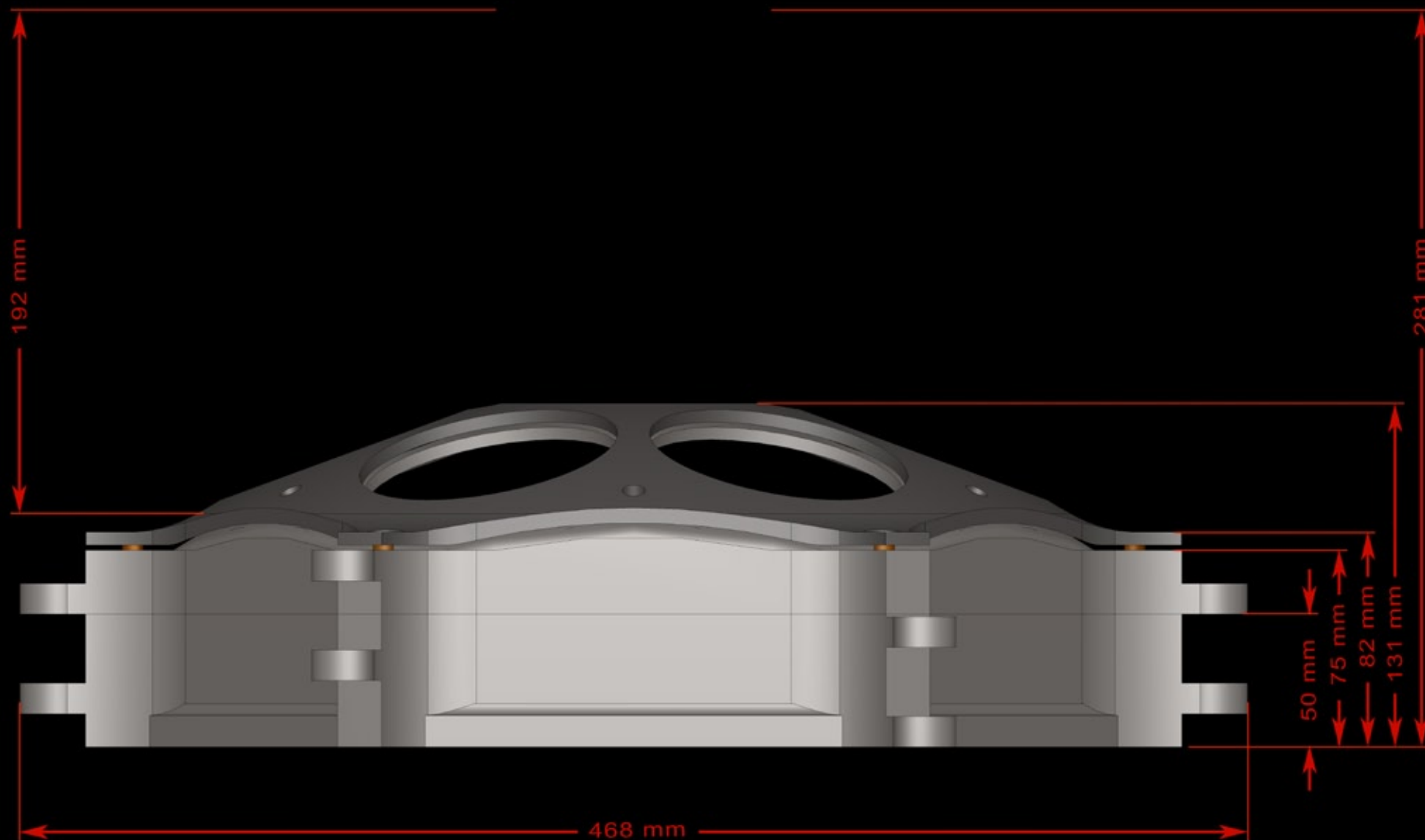
FLOWER HEAD CASING WITHOUT NOZZLE COVER
