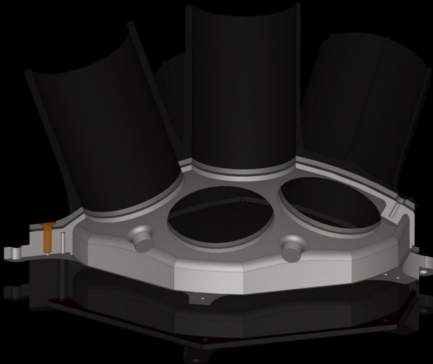
FLOWER HEAD CASING UPPER PART + COVER PLATE . PERSPECTIVE VIEW FROM BELOW
