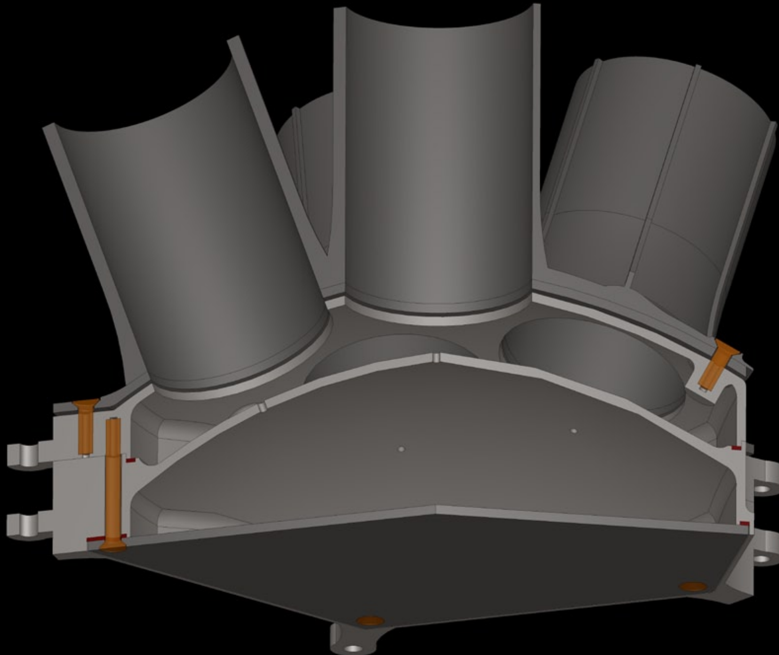
FLOWER HEAD COMPLETE . PERSPECTIVE VIEW FROM BELOW
