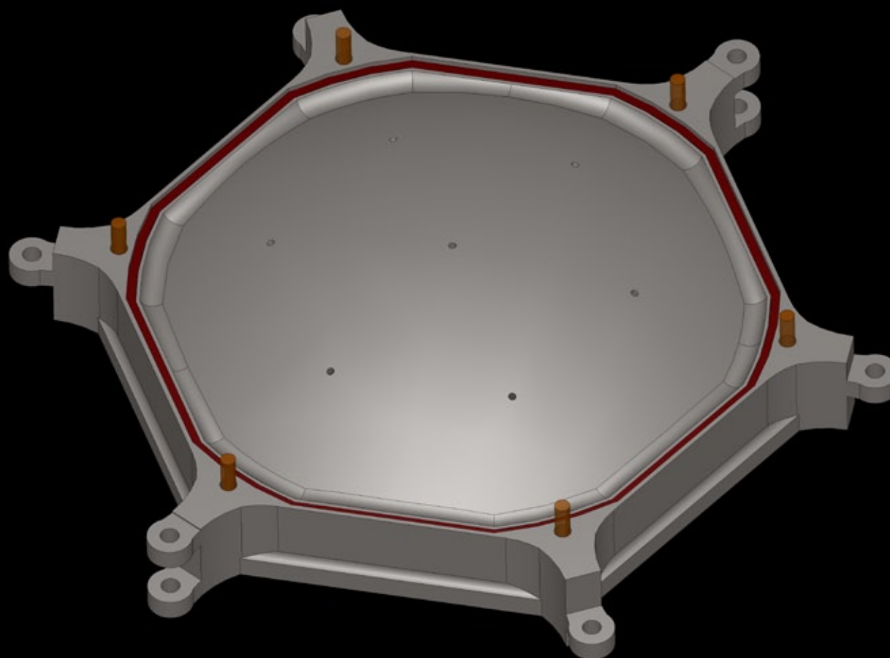
FLOWER HEAD CASING LOWER PART WITH GASKET
