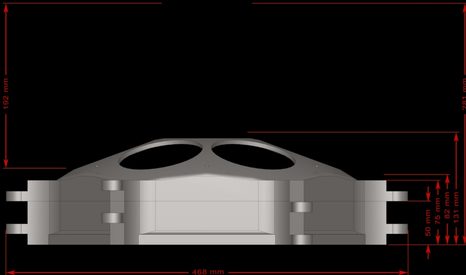
FLOWER HEAD CASING WITHOUT COVERPLATE AND NOZZLE COVER
