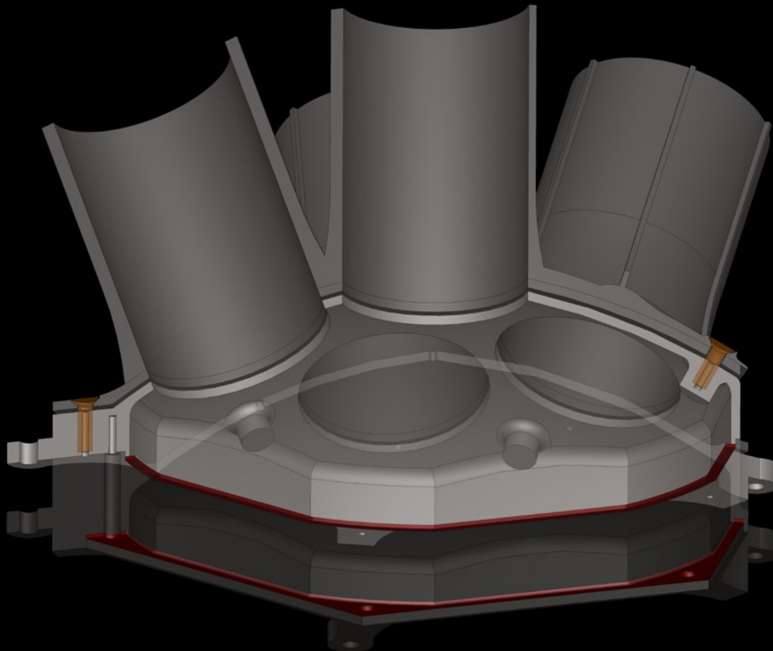
FLOWER HEAD UPPER PART . PERSPECTIVE VIEW FROM BELOW
