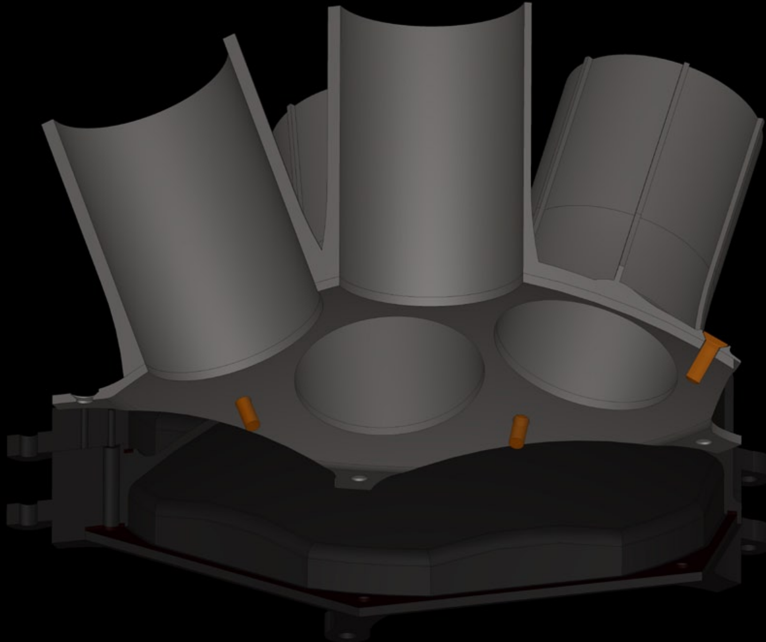
FLOWER HEAD COVER PLATE + NOZZLE COVER . PERSPECTIVE VIEW FROM BELOW
