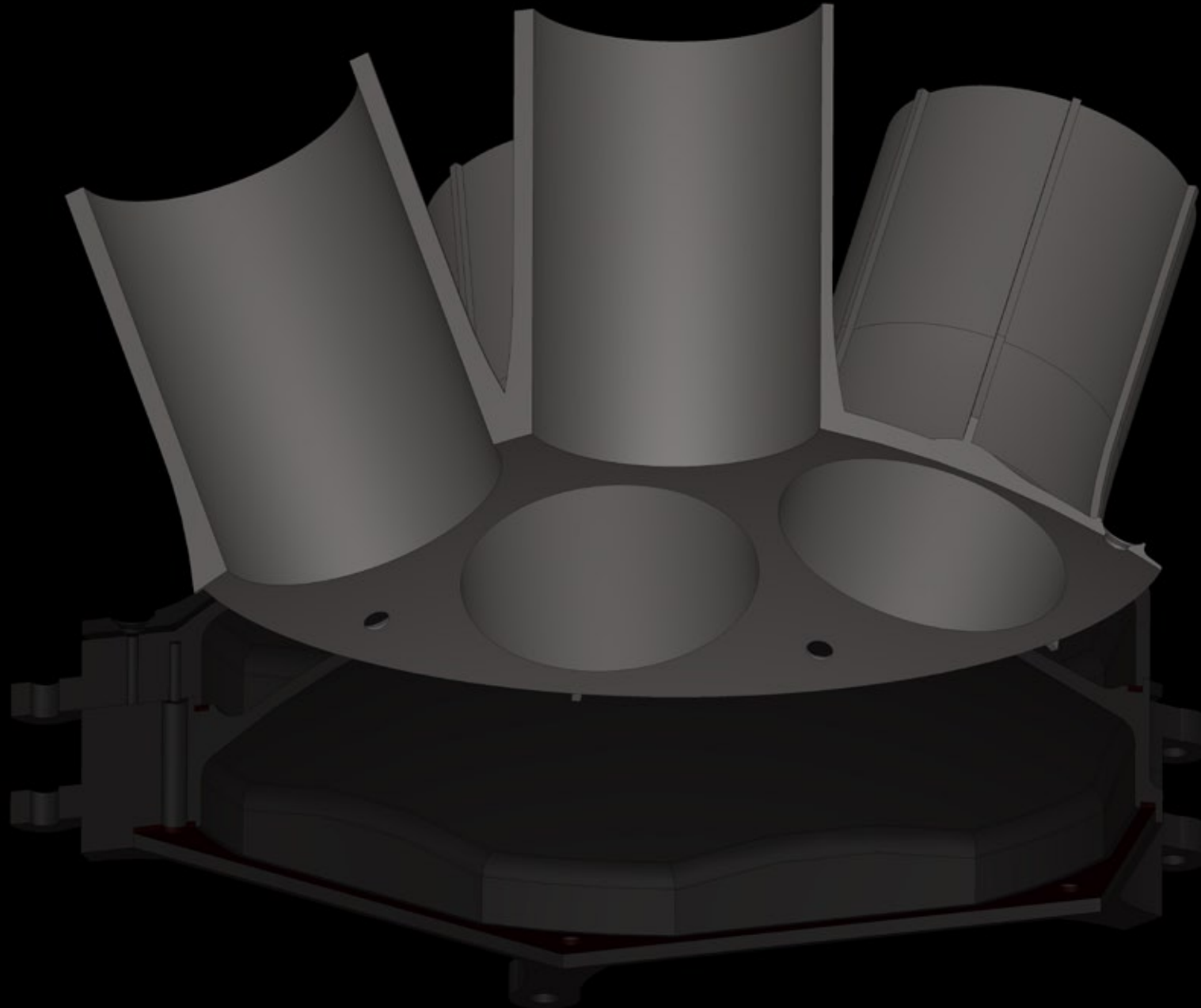
FLOWER HEAD NOZZLE COVER . PERSPECTIVE VIEW FROM BELOW
